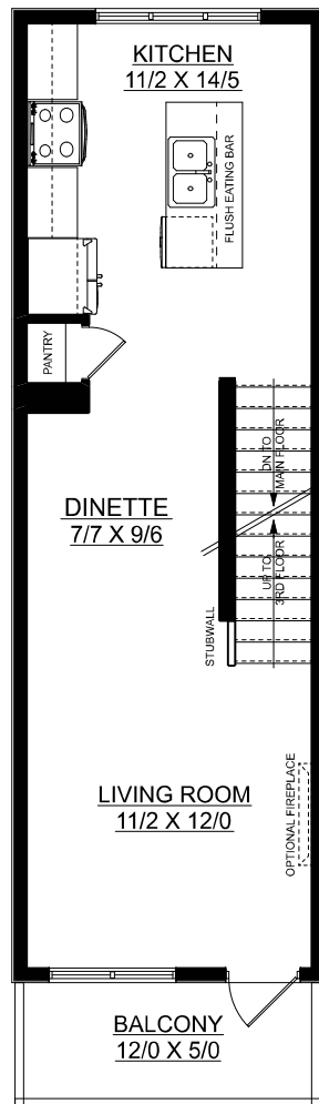
SECOND FLOOR PLAN 456 SQ. FT.
