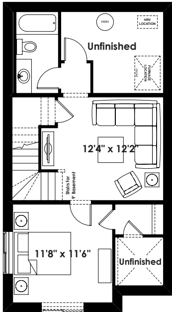
Optional 1 Bedroom Basement Room Layout With Dropped Entry (Southfork Only) 439 Sq. Ft. (Finished)
