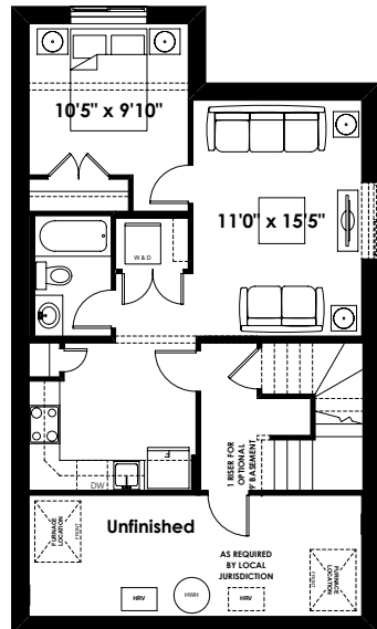
Optional Basement Suite Layout 597 Sq. Ft. (Finished Area; Must Add Optional Side Entry)
