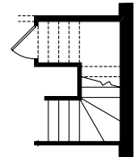
Partial Foundation Plan for Optional Side Entry (Lot & Bylaw Permitting; Stair Winders Relocated to Opposite Side of Stair)
