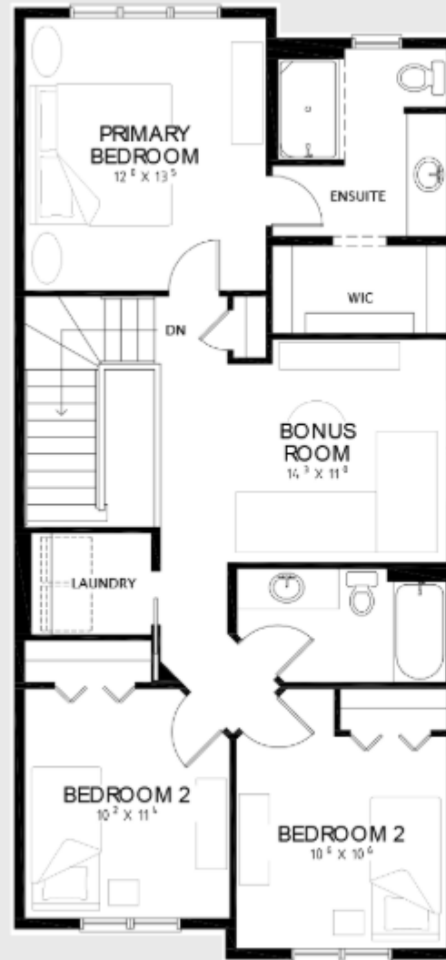
Upper Floor 984 Sq. Ft.
