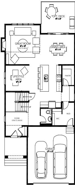
OPT. MAIN LEVEL 3 - Alternate Kitchen & Stairs 1236 SQ FT
