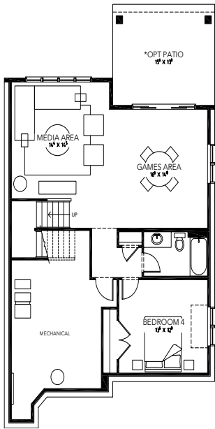
OPT. LOWER LEVEL 828 SQ FT
