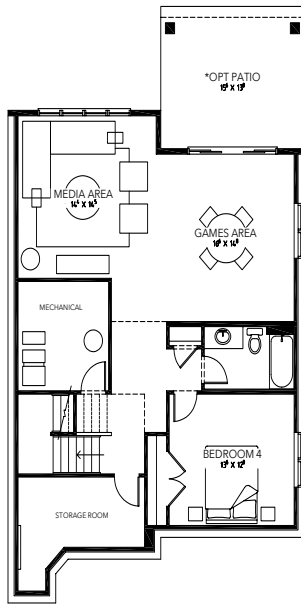
OPT. LOWER LEVEL 2 884 SQ FT
