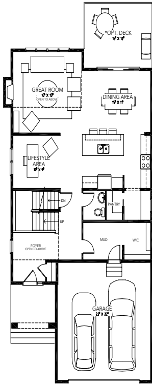
OPT. MAIN LEVEL 2 - Alternate Stairs 1236 SQ FT
