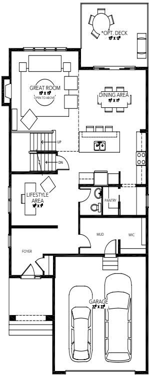
MAIN LEVEL 1236 SQ FT
