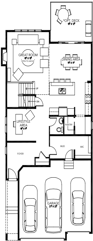
MAIN LEVEL 1248 SQ FT
