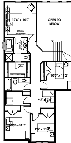
Optional Second Floor Plan with 4 Bedrooms, Tech Centre and Upper Floor Laundry Room for Caldwell - Base Elevation (Adds 0 Sq. Ft. to Second Floor)
