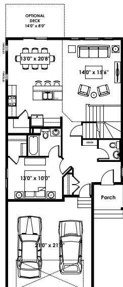
Main Floor Plan with Optional Main Floor Bedroom with Walk-in Closet, 3 Piece Ensuite and Powder Room for Caldwell - Base Elevation (Adds 11 Sq. Ft. to Main Floor)
