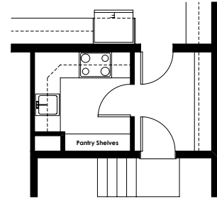
Partial Main Floor Plan with Optional Spice Kitchen (Adds 0 Sq. Ft. to Main Floor)
