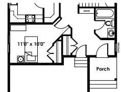
Partial Main Floor Plan with Optional Main Floor Bedroom & 3 Piece Bathroom (Adds 19 Sq. Ft. to Main Floor; Only Available with Expanded Spice Kitchen 2)
