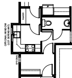
Partial Main Floor Plan with Optional Expanded Spice Kitchen (Adds 16 Sq. Ft. to Main Floor)
