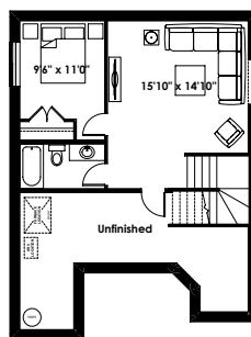
Optional Basement Room Layout for Optional Extended Garage 497 Sq. Ft. (Finished Area)
