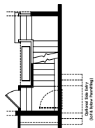
Partial Main Floor Plan with Optional Side Entry (Adds 0 Sq. Ft. to Main Floor; Lot & Bylaw Permitting) NOTE: BASEMENT STAIR UNFINISHED
