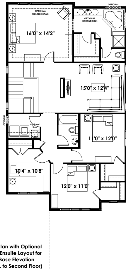
Partial Second Floor Plan with Optional Ensuite Layout (Adds 8 Sq. Ft. to Second Floor)
