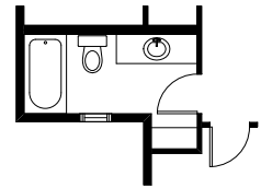
Partial Second Floor Plan with Optional Main Bath Vanity Extension (Adds 0 Sq. Ft. to Second Floor)
