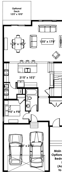
Main Floor Plan With Optional Bedroom & 3 Piece Bathroom (Adds 19 Sq. Ft. to Main Floor)
