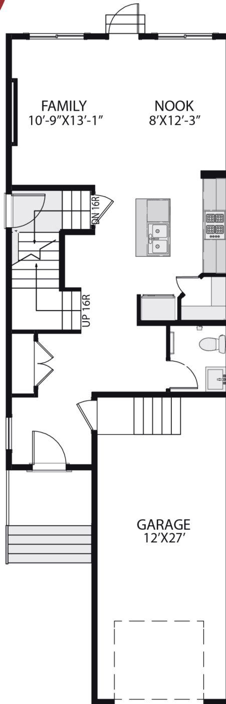
Main Floor 700 sqft.
