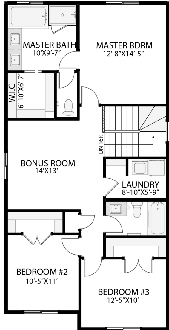
Upper Floor 1121 sqft.
