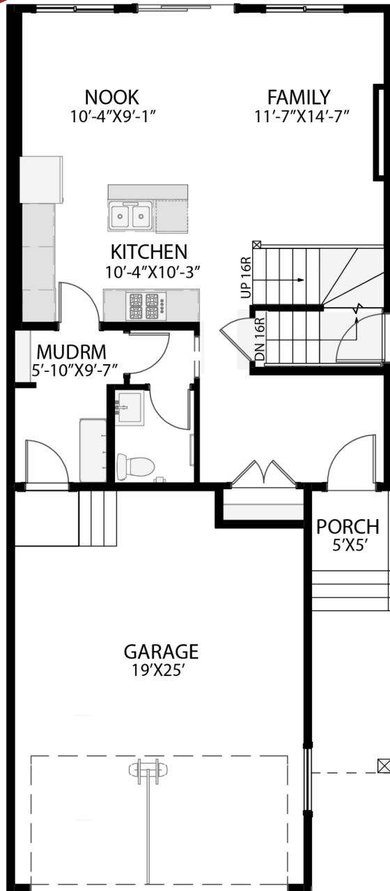
Main Floor 729 sqft.
