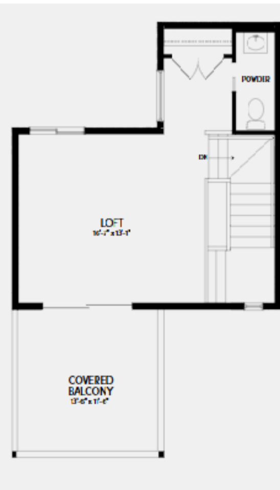
Third Level
