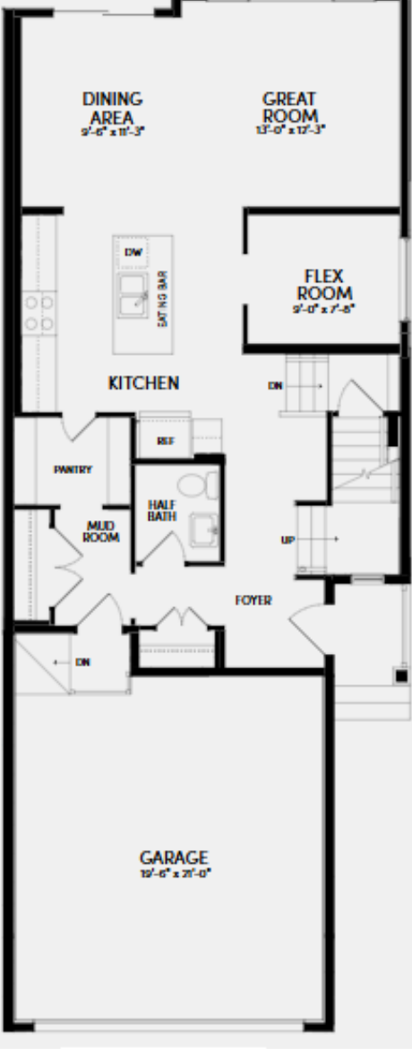
Main Level
