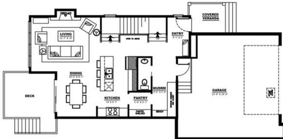
MAIN FLOOR PLAN = 795 SQ FT
