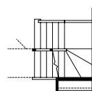
Partial Main Floor Plan with Optional Finished Stair to Basement c/w Center Wall Opening (Adds 0 Sq. Ft. to Main Floor)
