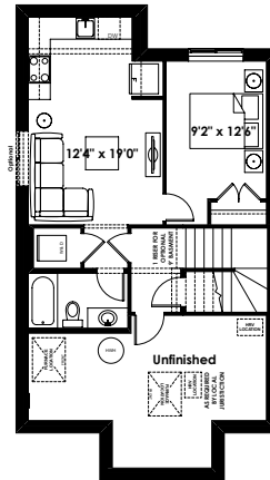
Optional Basement Suite Layout with Extended Kitchen Options 532 Sq. Ft. (Finished Area)
