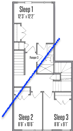
ALT. THIRD FLOOR (LOFT)
