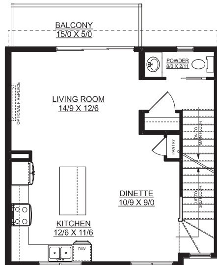
SECOND FLOOR PLAN 591 SQ. FT.
