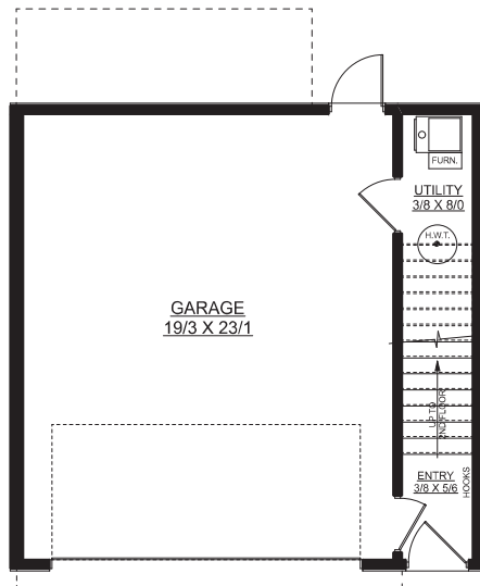
MAIN FLOOR PLAN 61 SQ. FT.
