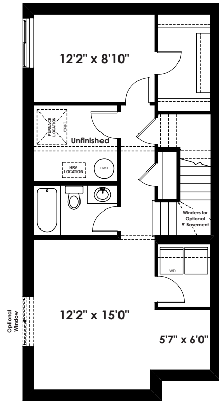
Optional Basement Room Layout For Optional Side Entry 583 Sq. Ft. (Finished)
