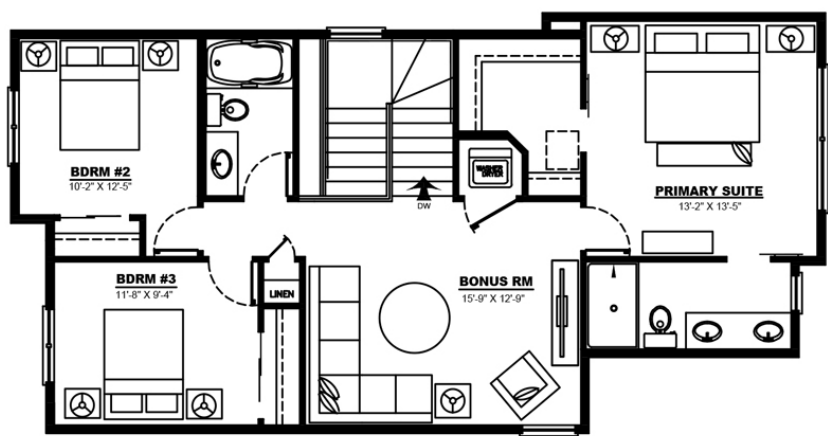
UPPER FLOOR PLAN = 993 SQ FT
