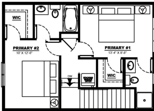
2 BED UPPER FLOOR = 560 SQ FT
