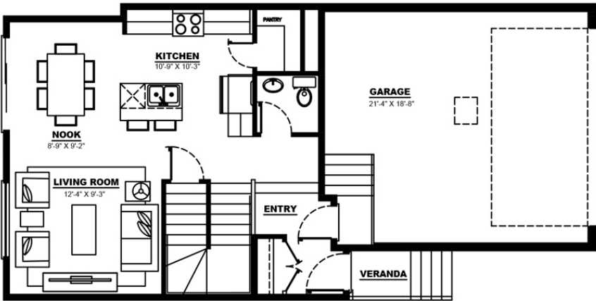
MAIN FLOOR PLAN = 619 SQ FT
