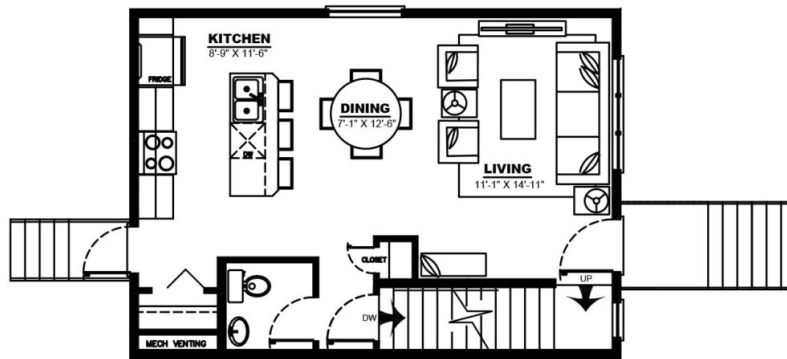
MAIN FLOOR PLAN = 481 SQ FT
