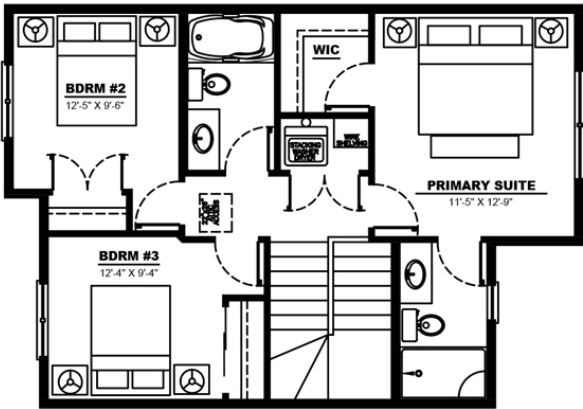
UPPER FLOOR PLAN = 688 SQ FT
