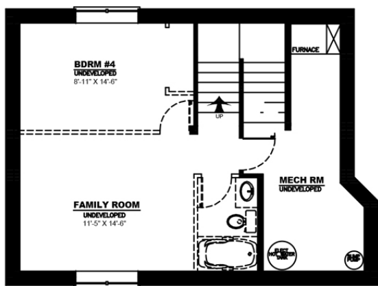
LOWER FLOOR PLAN = 498 SQ FT
