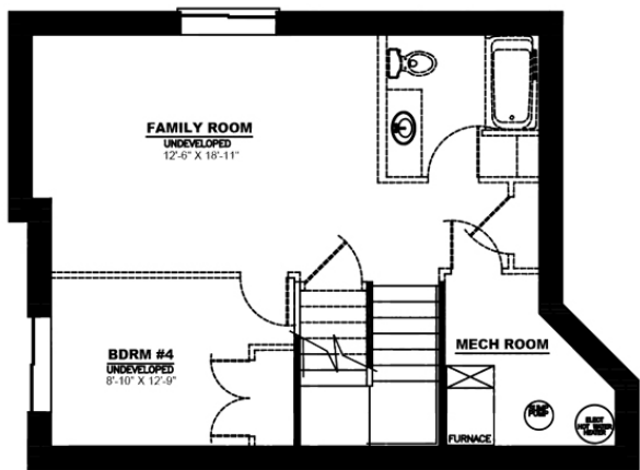
LOWER FLOOR PLAN = 415 SQ FT
