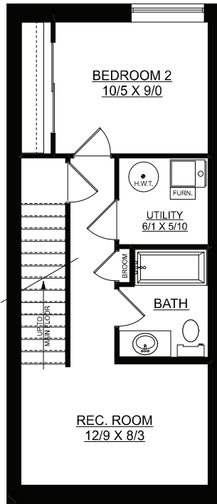
OPTIONAL BASEMENT PLAN 400 SQ. FT.
