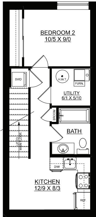
OPTIONAL BASEMENT SUITE 400 SQ. FT.
