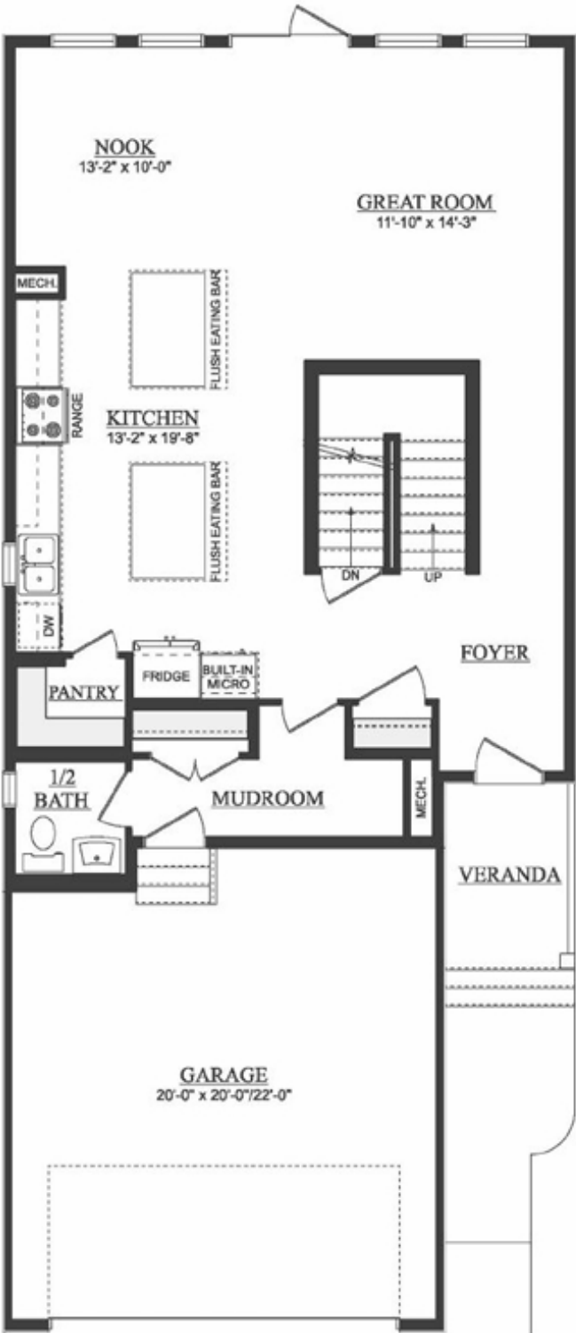
MAIN FLOOR PLAN 956 SQ. FT. (RMS)
