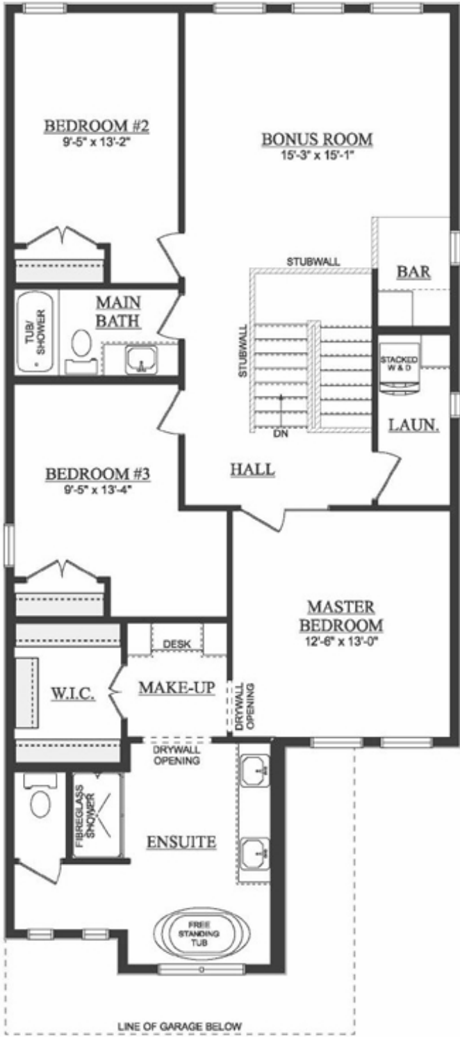
SECOND FLOOR PLAN 1300 SQ. FT. (RMS)
