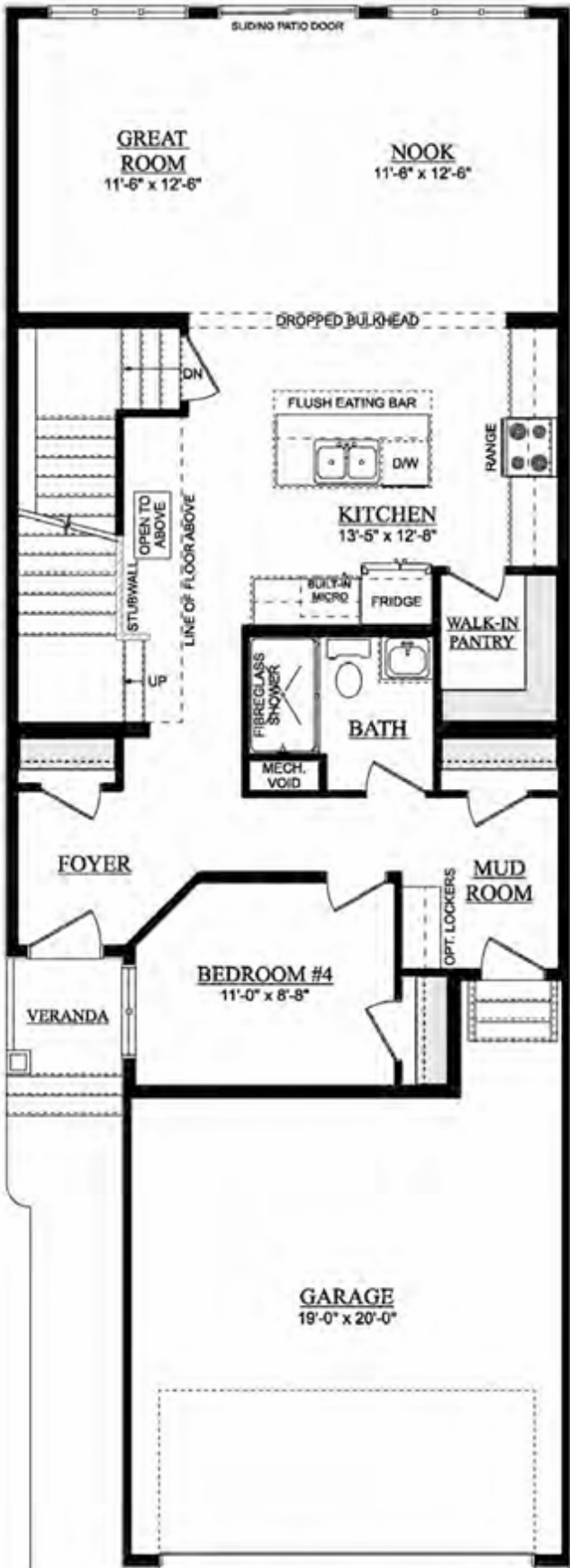
MAIN FLOOR PLAN 1062 SQ. FT. (RMS)
