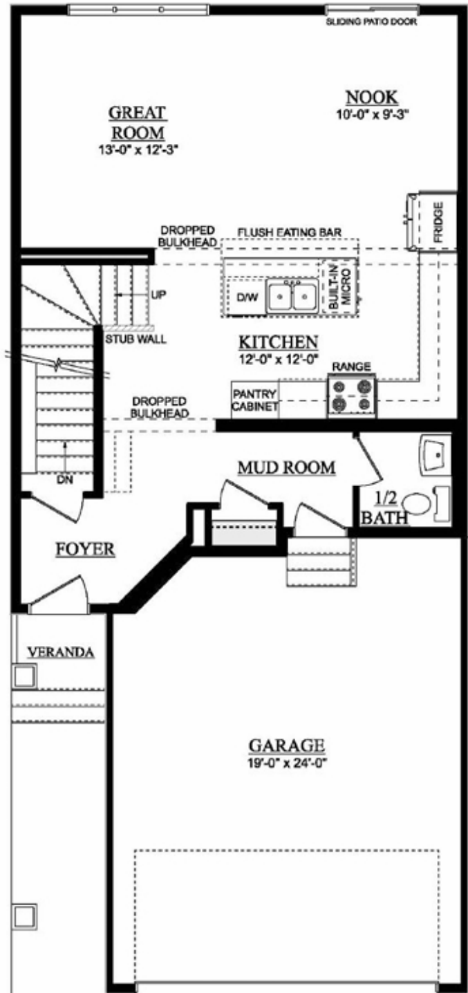
MAIN FLOOR PLAN 711 SQ. FT. (RMS)
