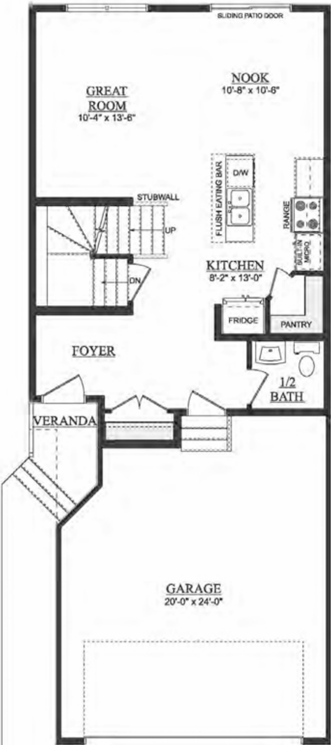
MAIN FLOOR PLAN 669 SQ. FT. (RMS)
