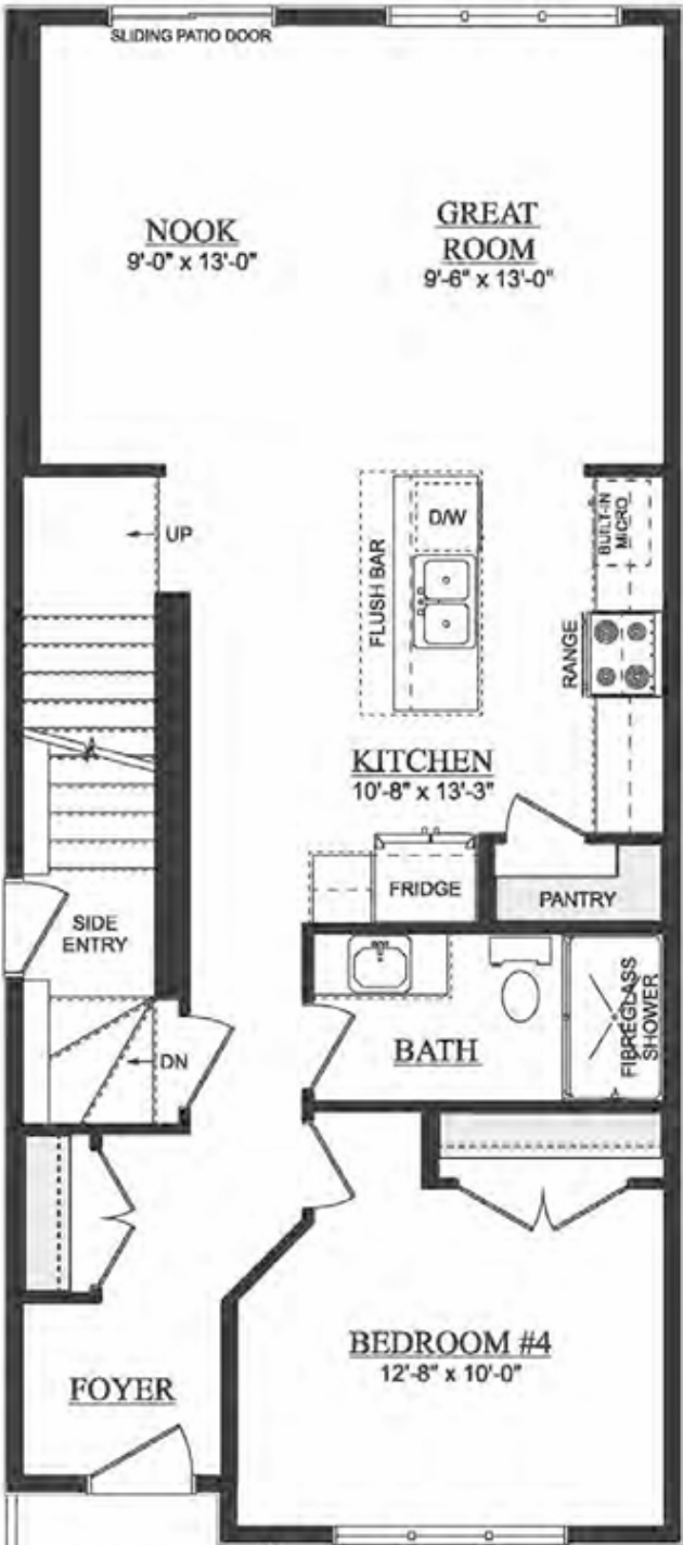
MAIN FLOOR PLAN 900 SQ. FT. (RMS)
