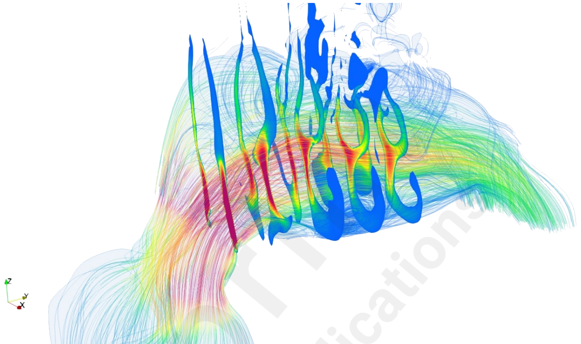
View of air flow with sections, scale up to 2.5 m/s
