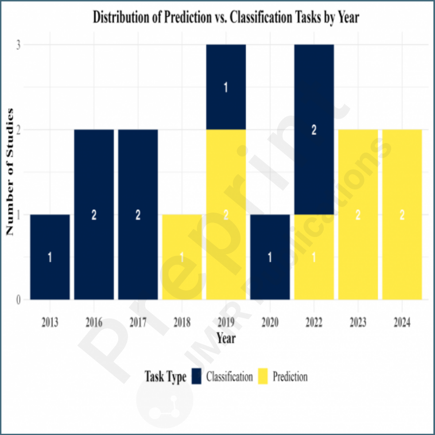
Distribution of Studies on Machine Learning and Deep Learning Applications for Leptospirosis Diagnosis and Prediction by Year and Task Type.
