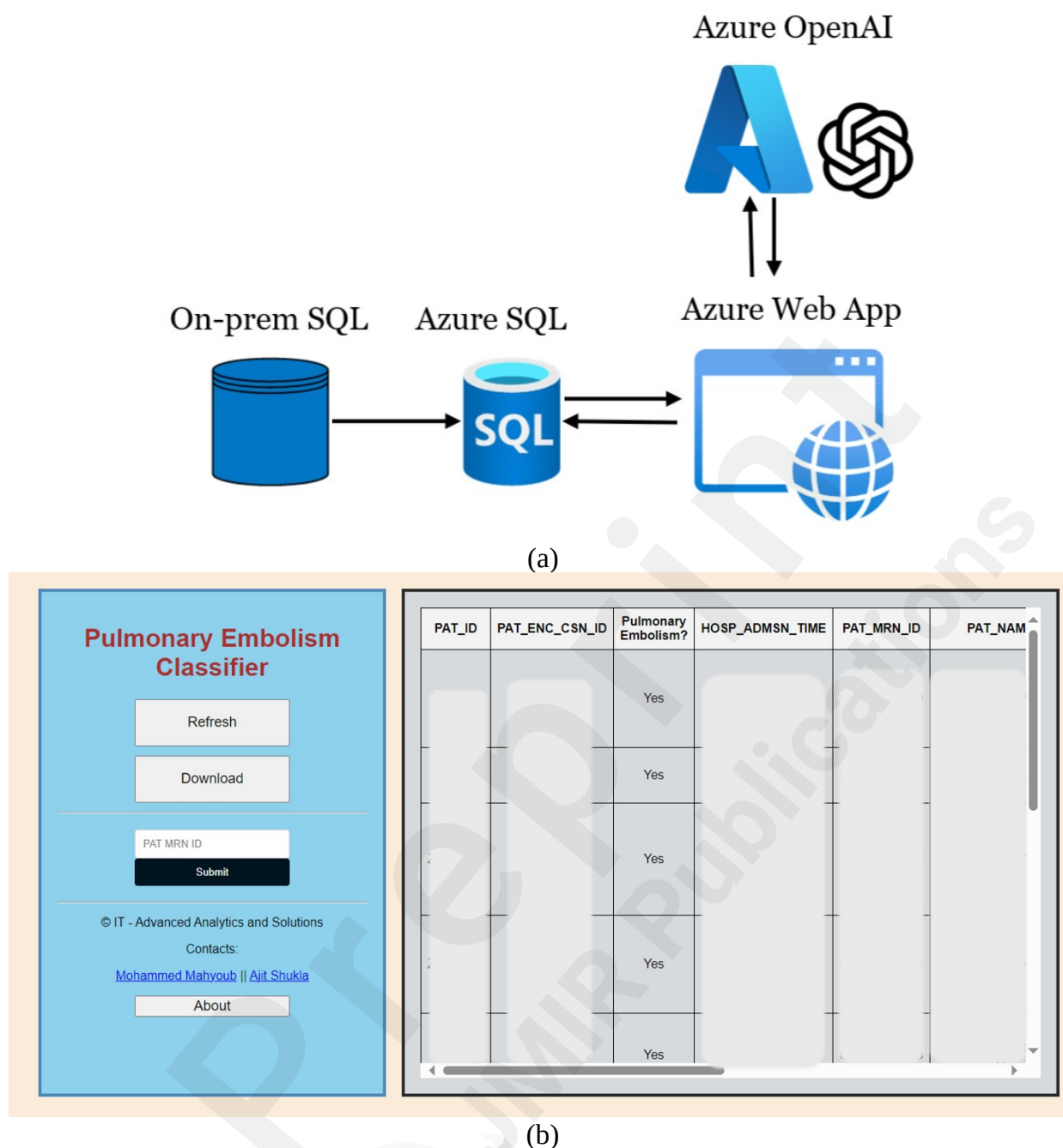
Figure 3. Deployment pipeline and consumption Web App. Only positive cases are displayed. This Web App has been operationalized at Virtua Health, NJ.
