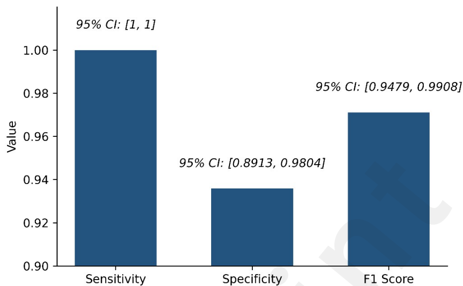
Figure 5. Post-deployment performance metrics of GPT-4o.
