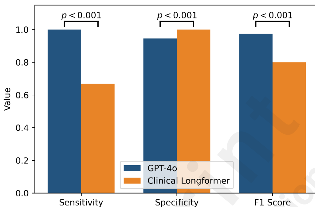
Figure 4. Evaluation metrics comparison of Clinical Longformer (baseline model) and GPT-4o.
