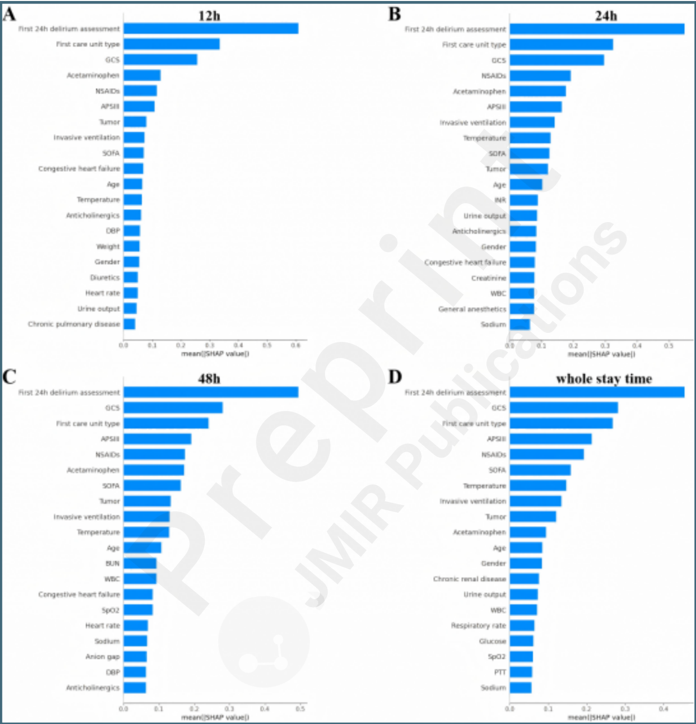
Feature importance ranking plot of the XGB machine learning models in different prediction windows (top 20 features).
