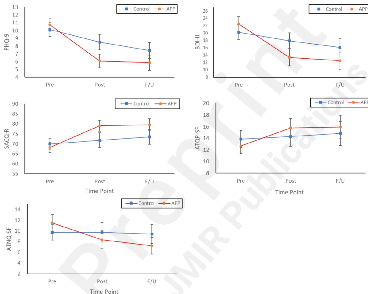
Figure 3. Means and 95% intervals for the groups across the assessment time points
