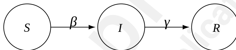
Figure 2: SIR model diagram showing compartments and flow.
